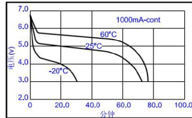
Discharge Characteristics at 1000mA
